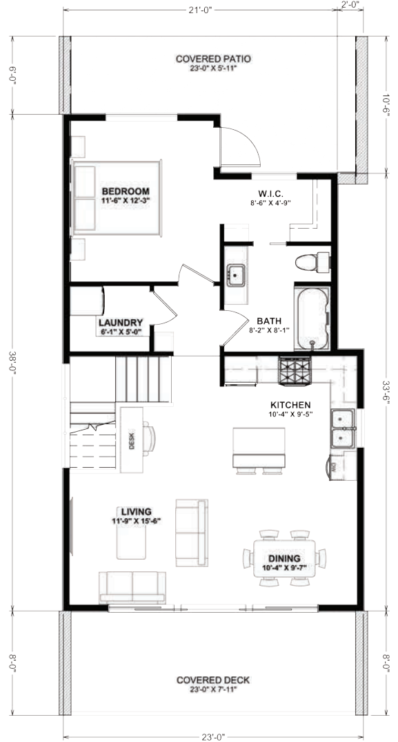
MAIN LEVEL (PLAN 9)
